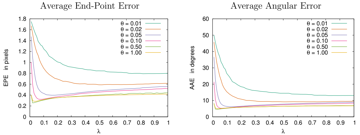
Figure 6: Errors for sequence "Yosemite with Clouds" as a function of \lambda .
